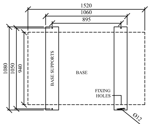
PLAN VIEW OF UNIT BASE
