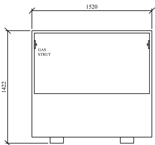
VIEW OF ACCESS OPENING - LID REMOVED
