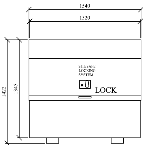
FRONT ELEVATION
