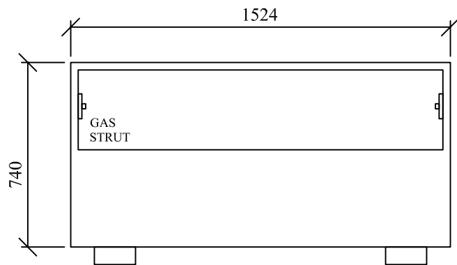
VIEW OF ACCESS OPENING - LID REMOVED
