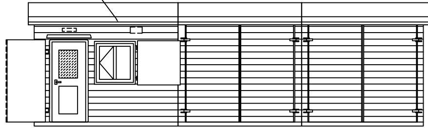
FRONT ELEVATION
