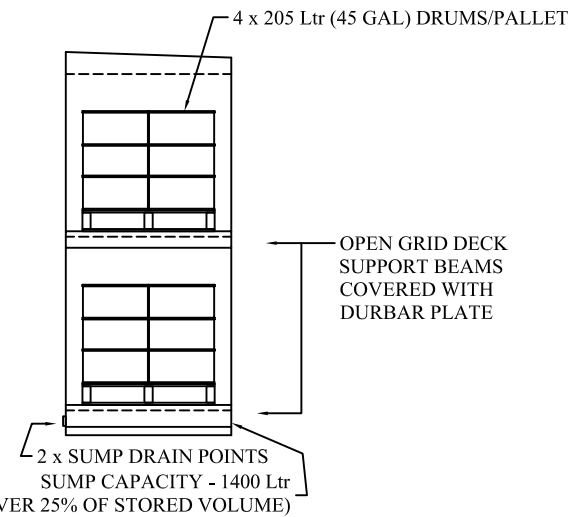
TYPICAL SECTION
