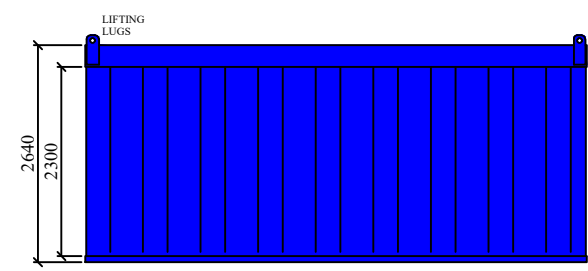
SIDE ELEVATION
